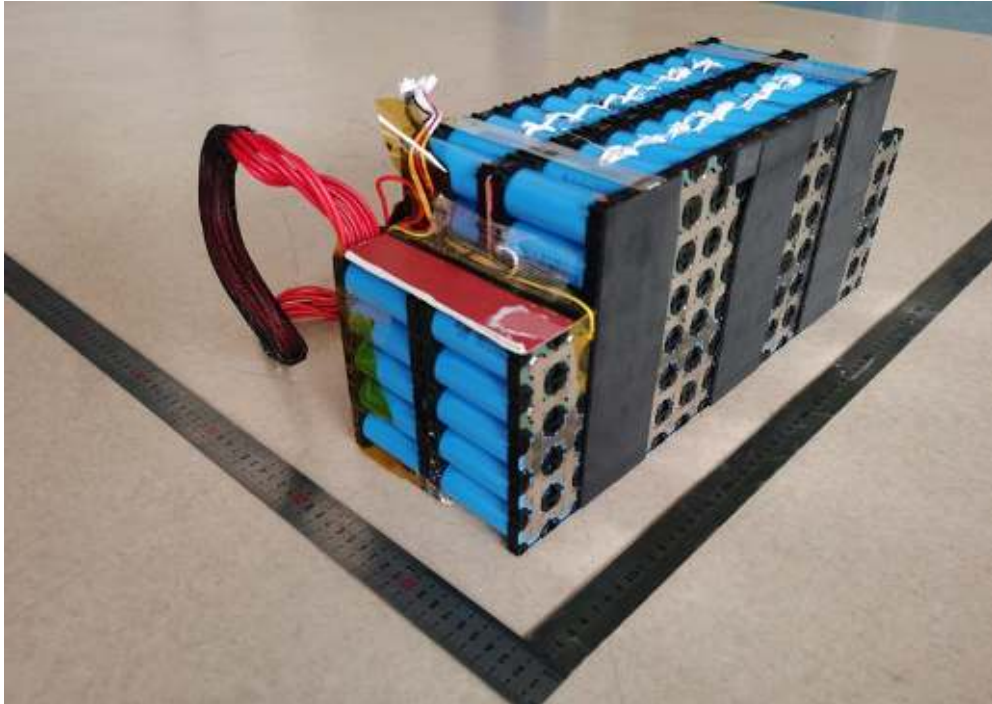
Internal view (Model No. HKPBATL240B)
