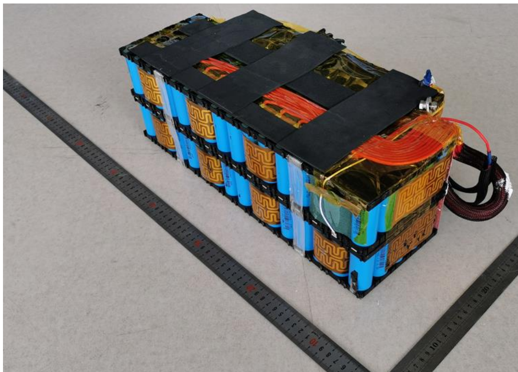
Internal view (Model No. HKPBATL240BH)
