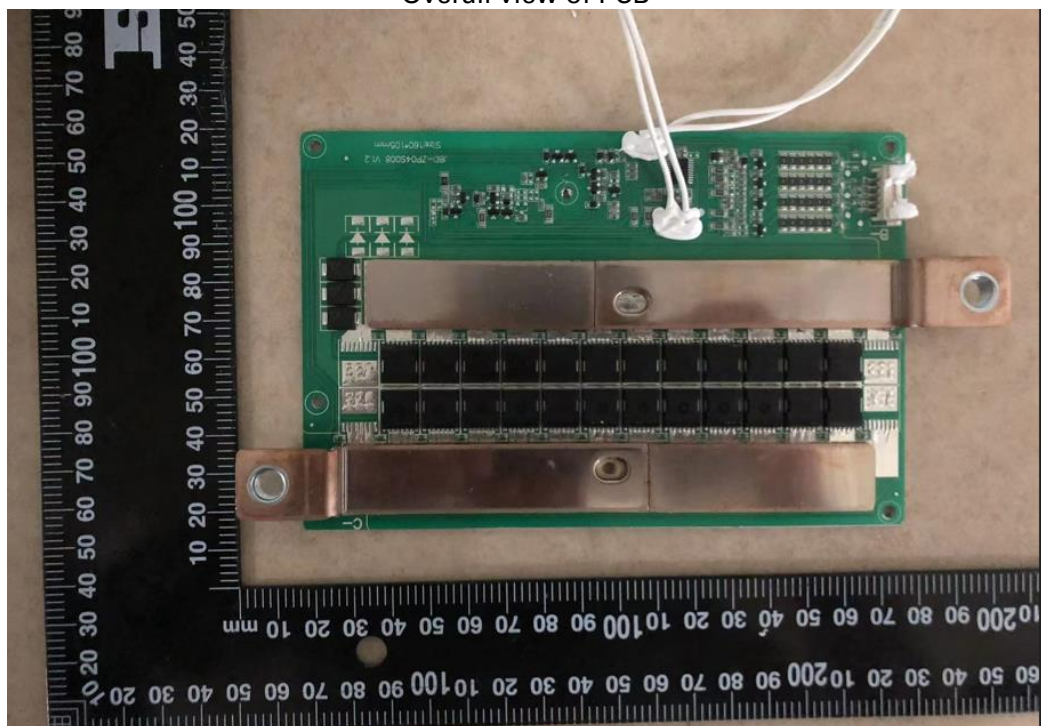
Overall view of PCB
