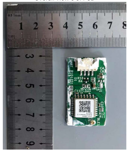
Overall view 3 of PCB
