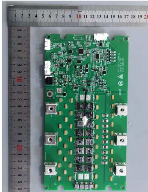
Overall view 1 of PCB
